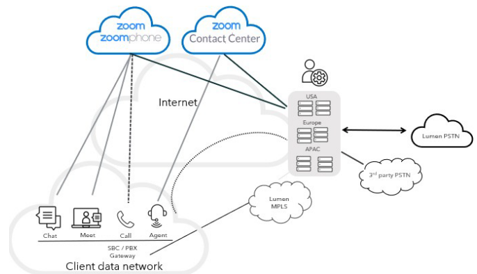
Figure 2 – Cloud peering with virtual SBCs
